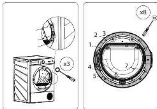
4. Remove inner glass from door
