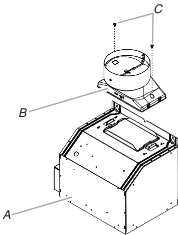
A. In-line housing B. Vent transition (with backdraft damper) C. 3.5 x 9.5 mm screws (2)
