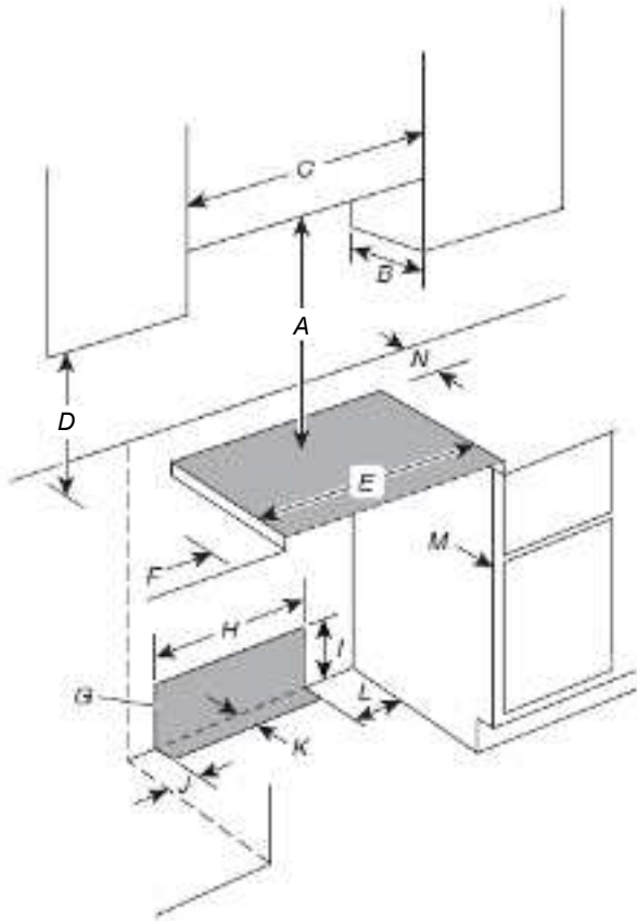
Slide-In Cutout
