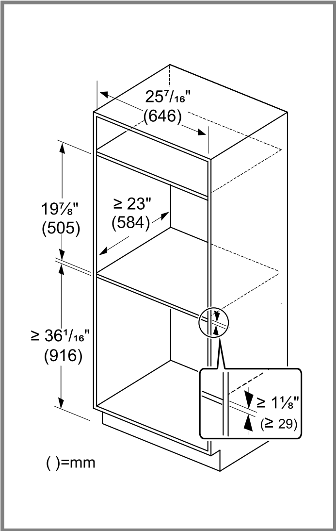
Cabinet dimensions for installation with 27" trim kit
