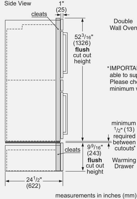
Flush Installation Double Oven over Storage or Warming Drawer
