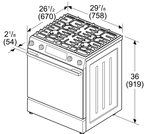
Measurements in inches (mm)
