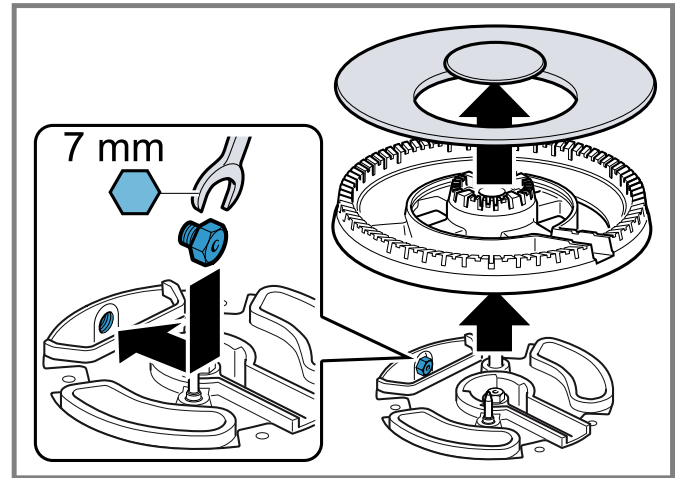
Double burner, first orifice
