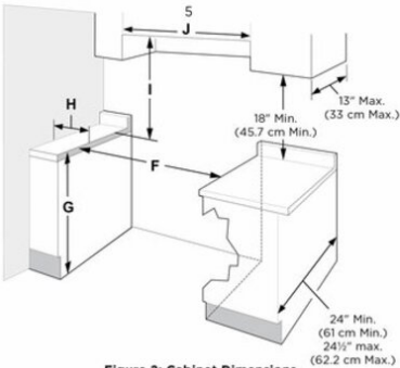
Figure 2: Cabinet Dimensions
