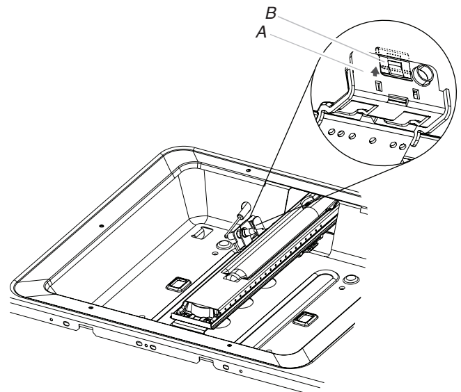
A. Oven bake burner electrode bracket
