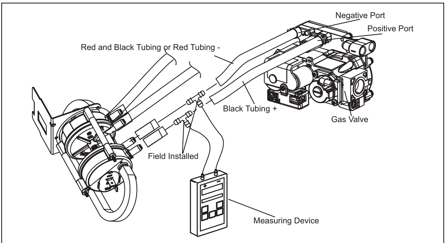
Figure 49. Operating Signal (Delta P) Measurement
