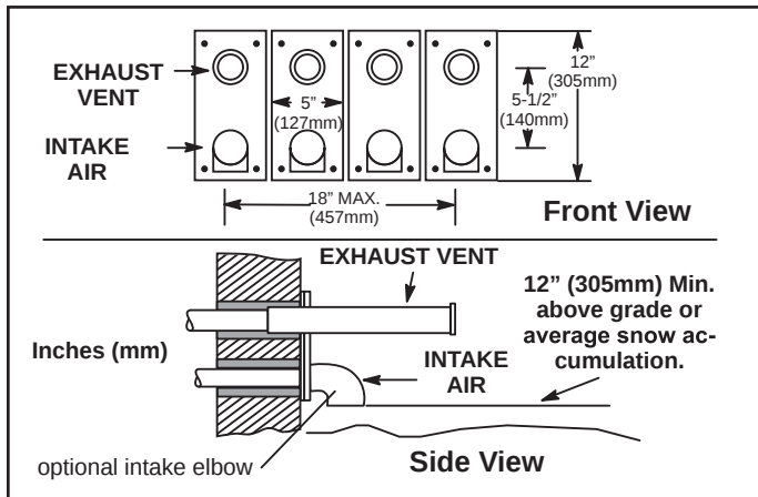
Figure 30. Optional Vent Termination for Multiple Unit Installation of Direct Vent Wall Termination
