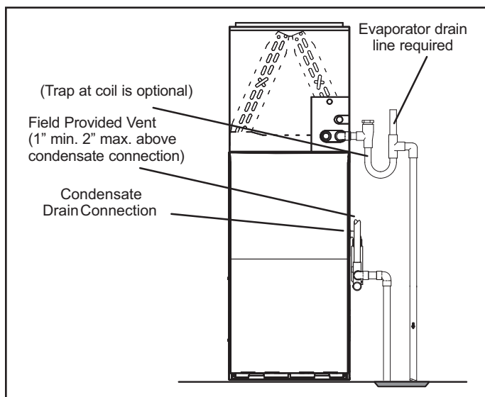
Figure 39. Furnace with Evaporator Coil Using a Separate Drain
