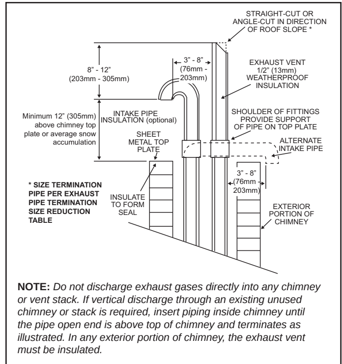
Figure 32. Direct Vent Application Using Existing Chimney
