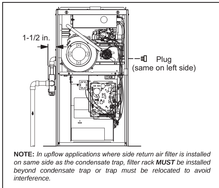
Figure 36. Condensate Trap and Plug Locations (Unit Shown in Upflow Position)
