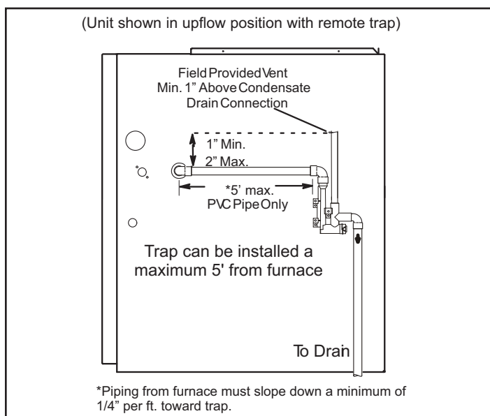
Figure 37. Condensate Trap Locations
