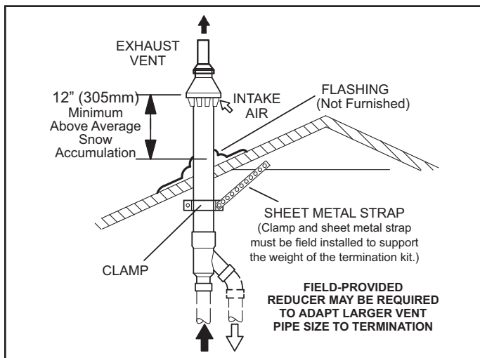
Figure 31. Direct Vent Concentric Rooftop Termination 71M80, 69M29 or 60L46 (US) 44W92 or 44W93 (Canada)
