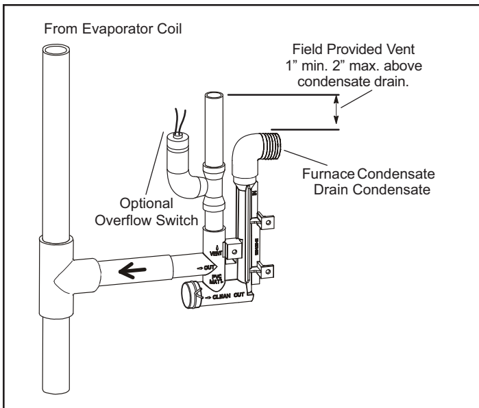
Figure 41. Condensate Trap With Optional Overflow Switch
