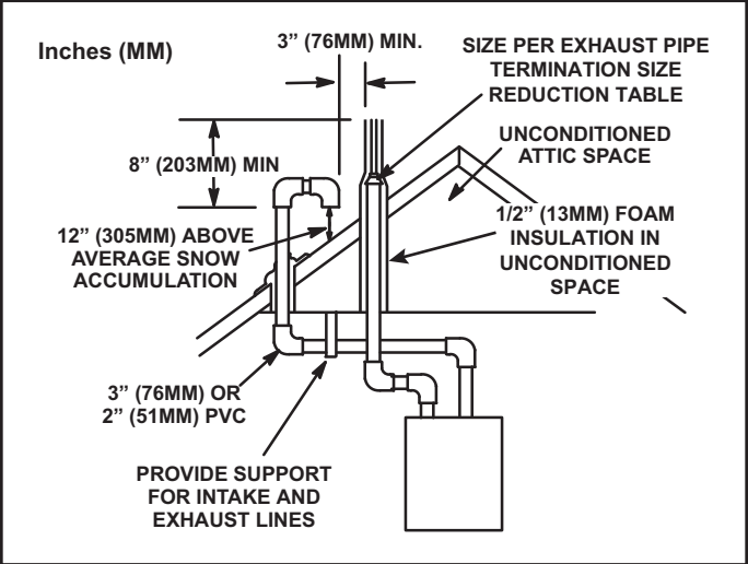
Figure 29. Direct Vent Roof Termination
