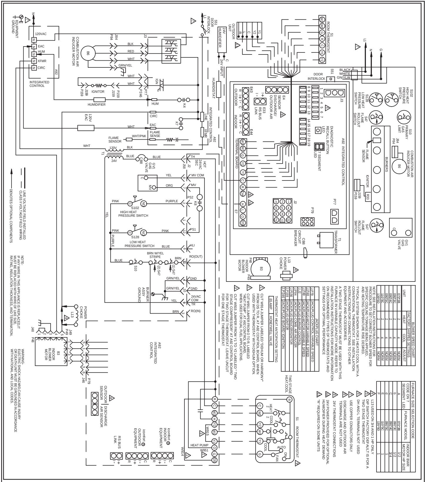
Figure 52. Typical Field Wiring
