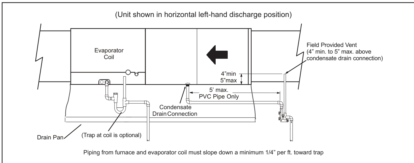
Figure 40. Furnace with Evaporator Coil Using a Separate Drain
