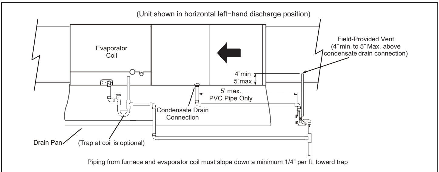
Figure 43. Furnace with Evaporator Coil Using a Common Drain
