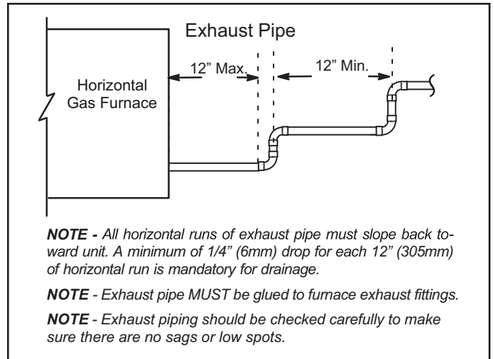
Figure 23. Horizontal Installation Offset Requirements
