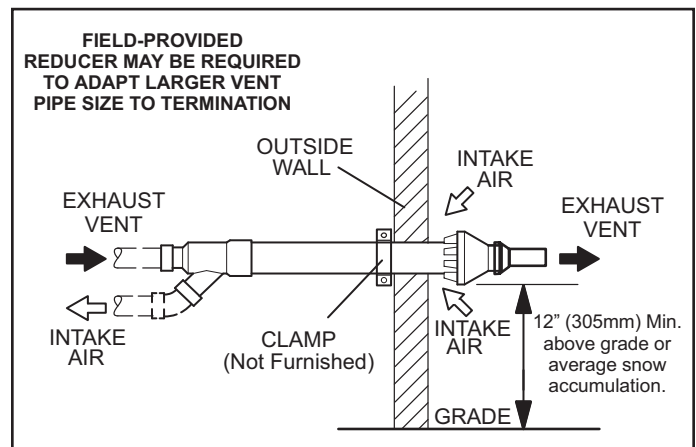
Figure 33. Direct Vent Concentric Wall Termination 71M80, 69M29 or 60L46 (US) 44W92 or 44W93 (Canada)
