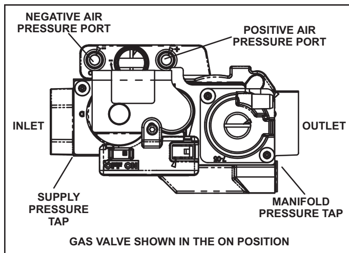
Figure 46. Gas Valve
