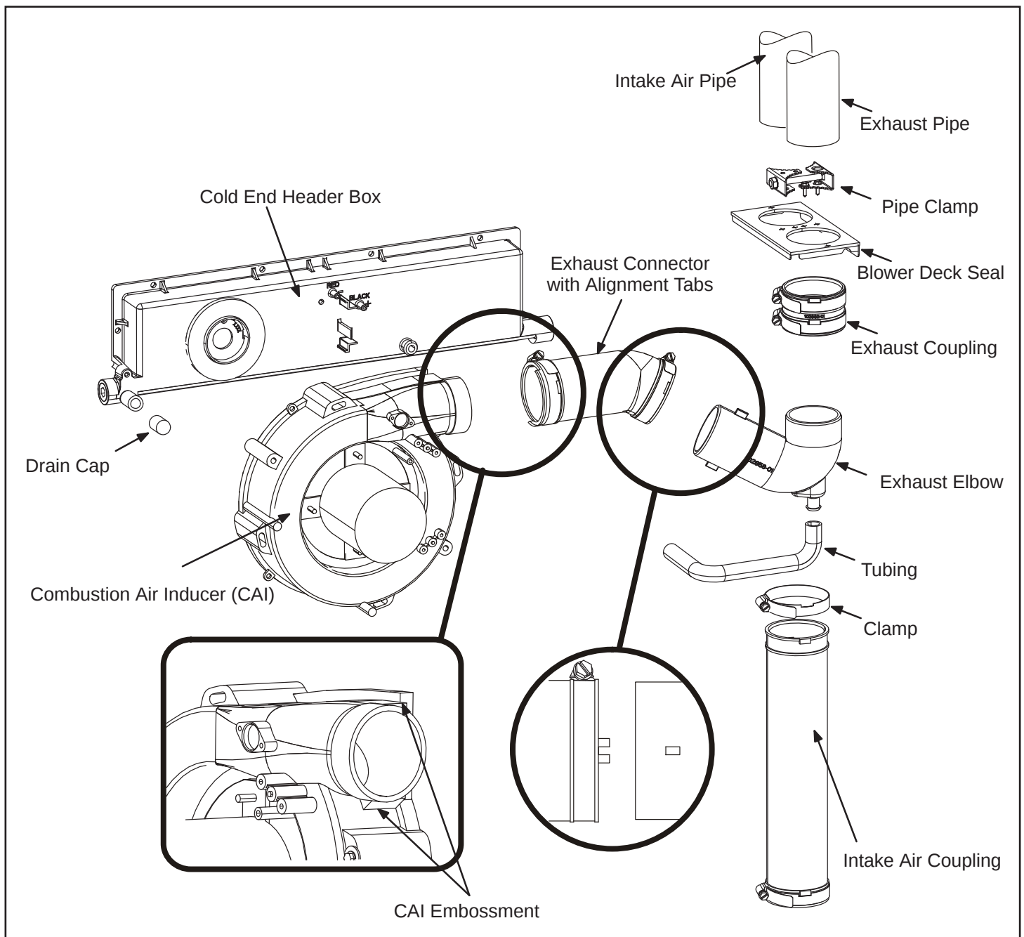
Figure 19. Combustion Air Inducer / Cold End Header Box / Vent Pipe Assembly
