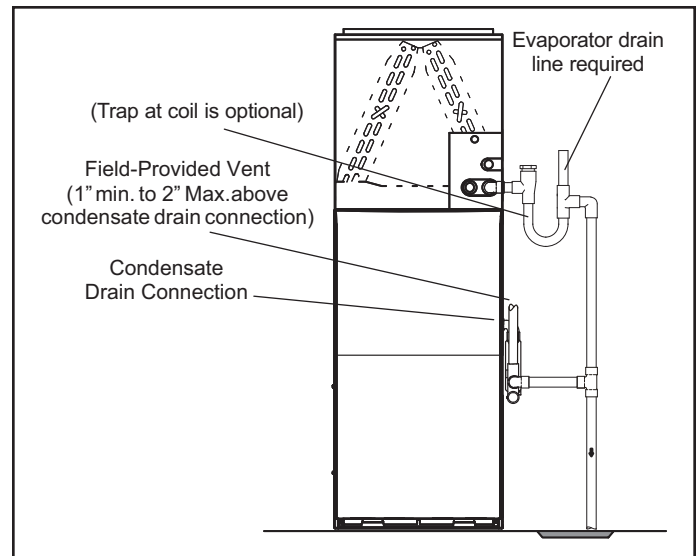
Figure 42. Furnace with Evaporator Coil Using a Common Drain
