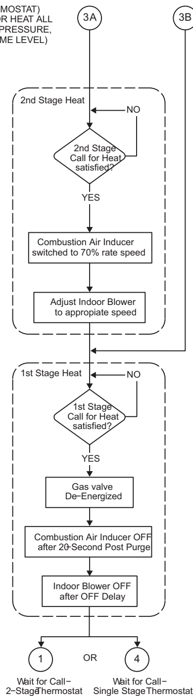
Figure 56. Call for Heat Satisfied
