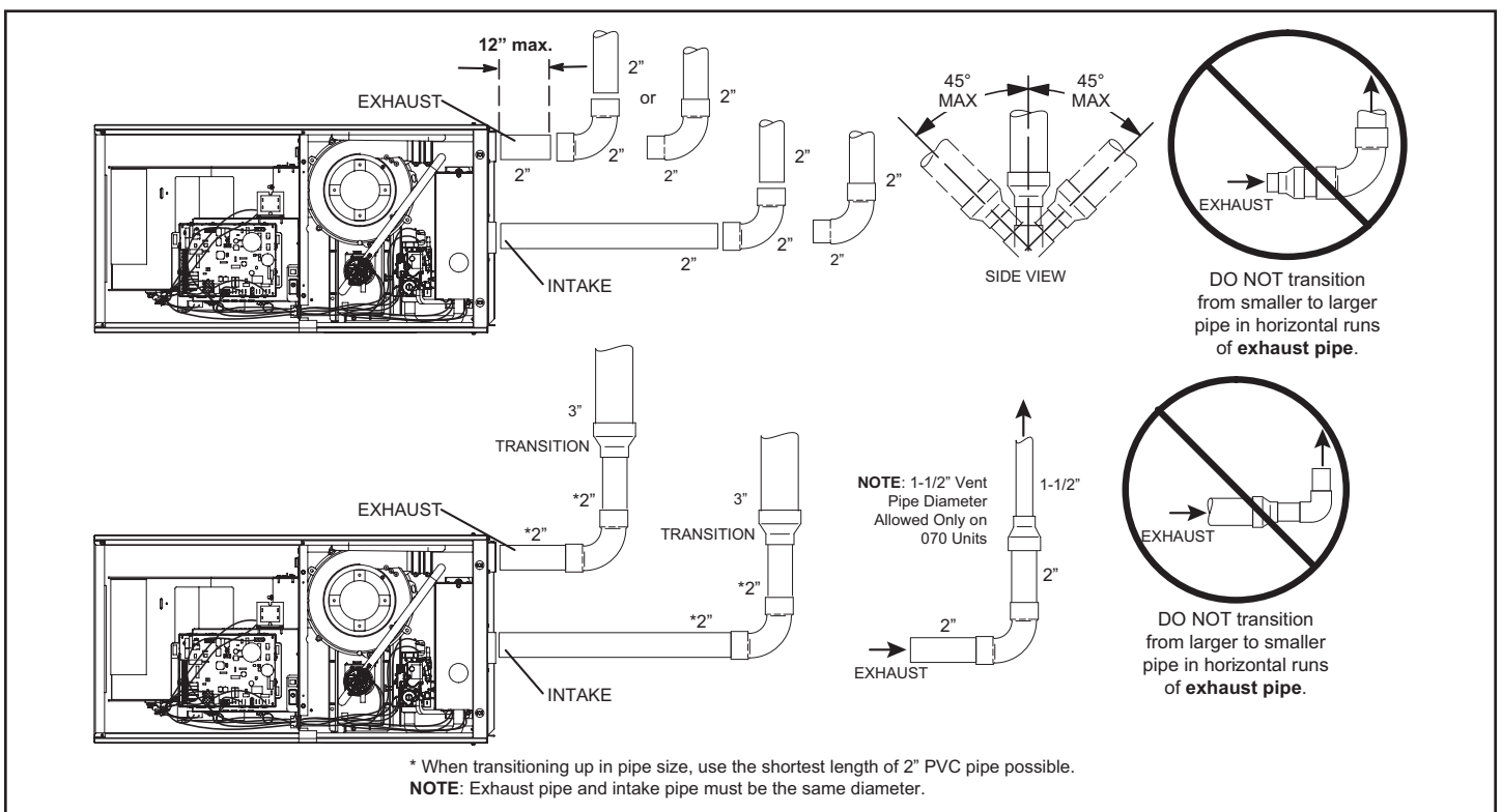
Figure 22. Typical Exhaust and Intake Pipe Connections and Condensate Trap Installation in Horizontal Air Applications (Right Hand Discharge Shown)
