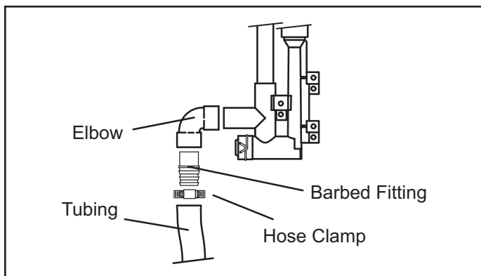
Figure 38. Field-Provided Drain Components
