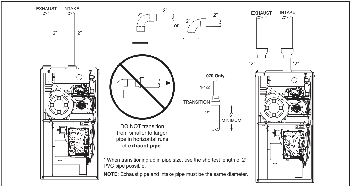
Figure 21. Typical Exhaust and Intake Pipe Connections and Condensate Trap Installation in Upflow Applications
