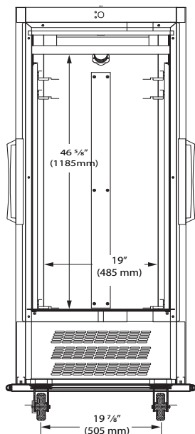
Front (Open)
