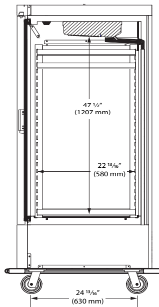
Side (Interior)
