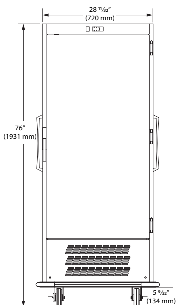
Front (Closed)
