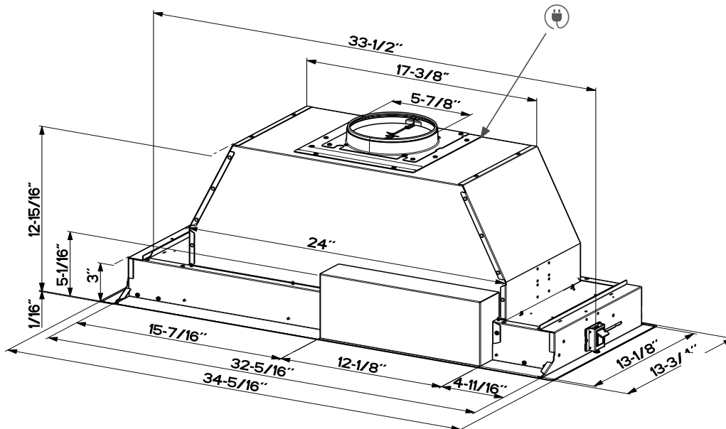
35" FRONT VIEW
