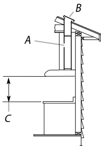
Roof venting
