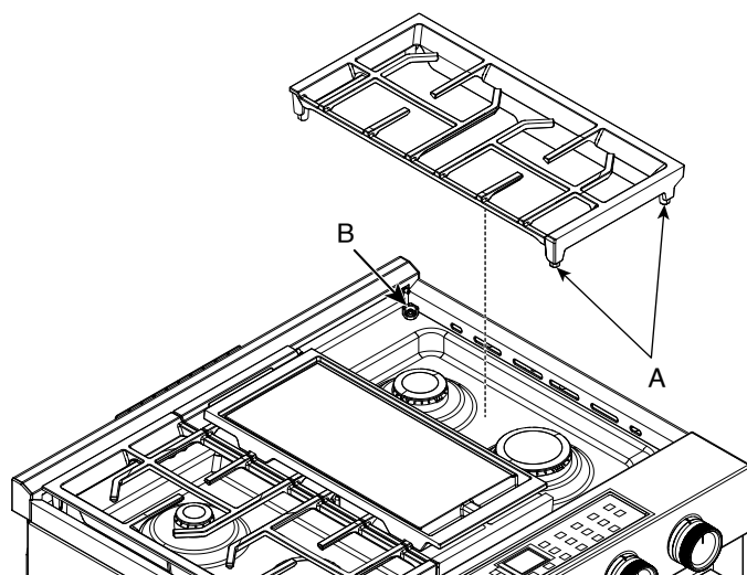
A. Bumpers B. Alignment indentations
