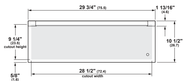
FRONT VIEW (SHOWING CUTOUT OVERLAP)
