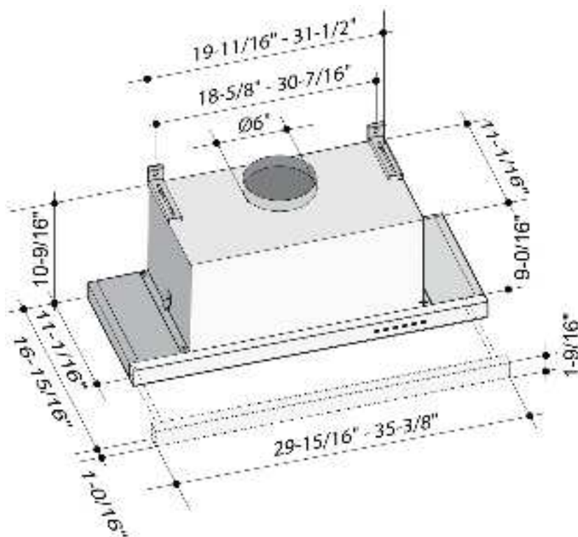
Cabinet Cutout Dimensions
