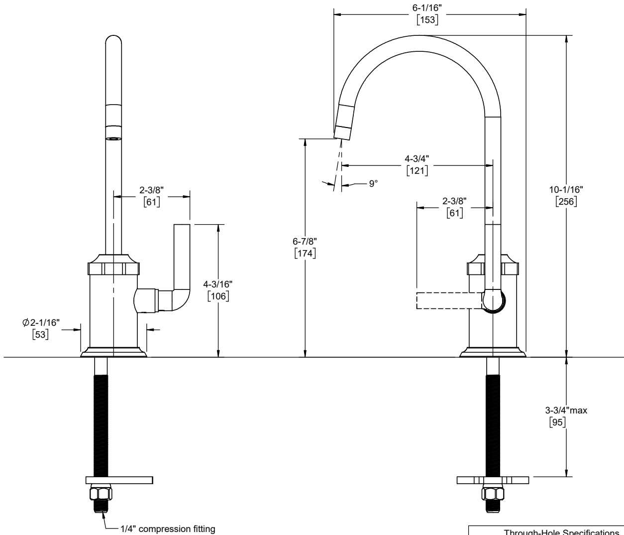
9620-K30-SL shown
