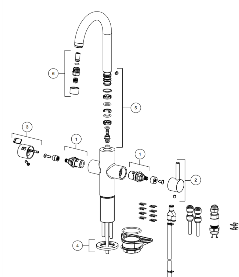
Tap Maris Lario Filtration&Boiling MB
