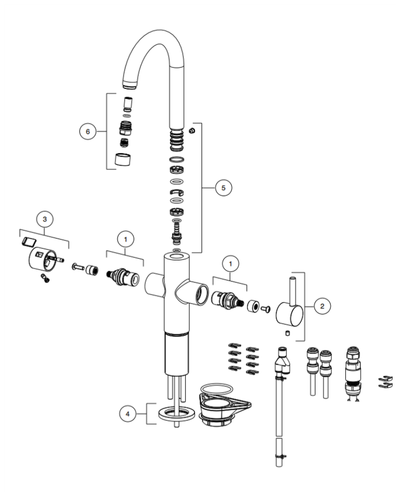
Tap Maris Lario Filtration&Boiling CHR
