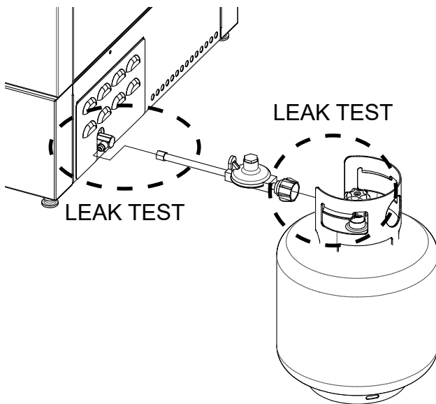
TYPICAL BOTTLE LP GAS HOOK-UP
