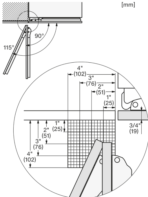
Hinge Details
