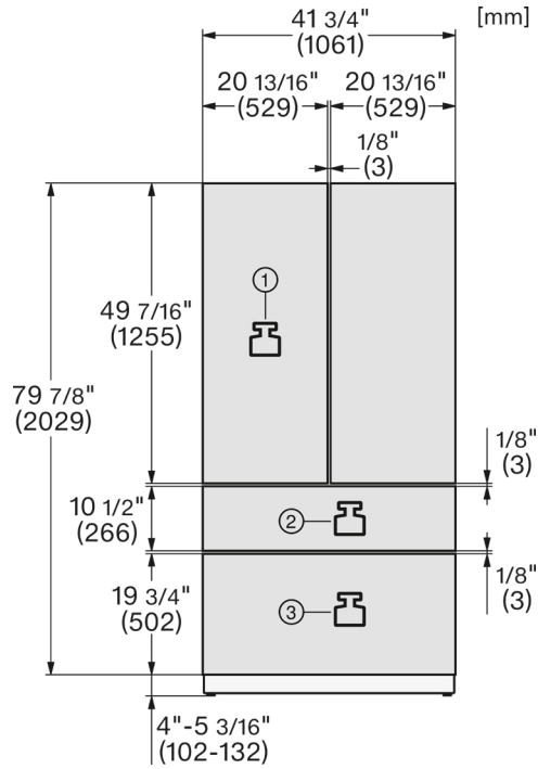
Panel Details
