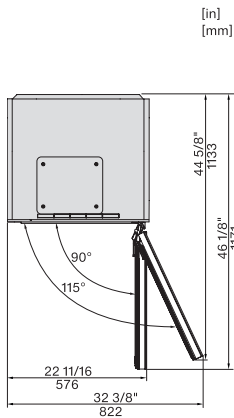
KWTUS7172F, Built-under, top view (installation drawings)
